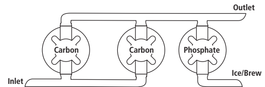
ex. Twin Head Parallel Flow with Scale Reduction
