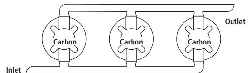
ex. Triple Head Parallel Flow
